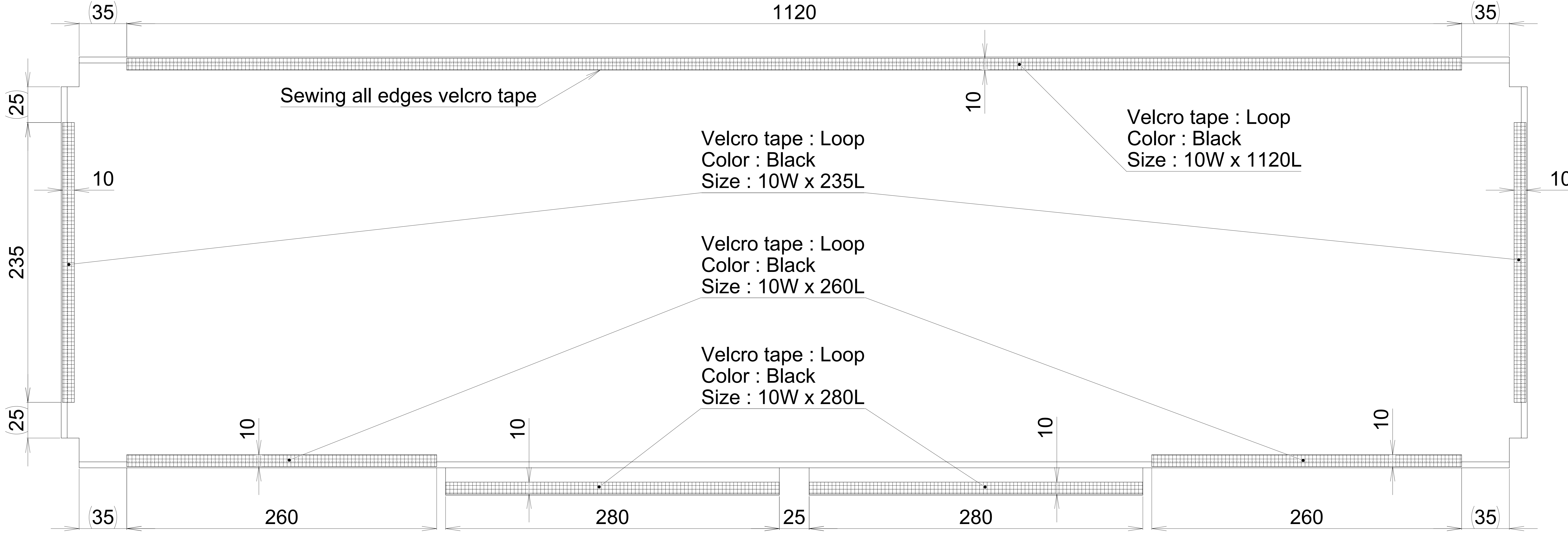
BACK (Velcro tape sewing position)
